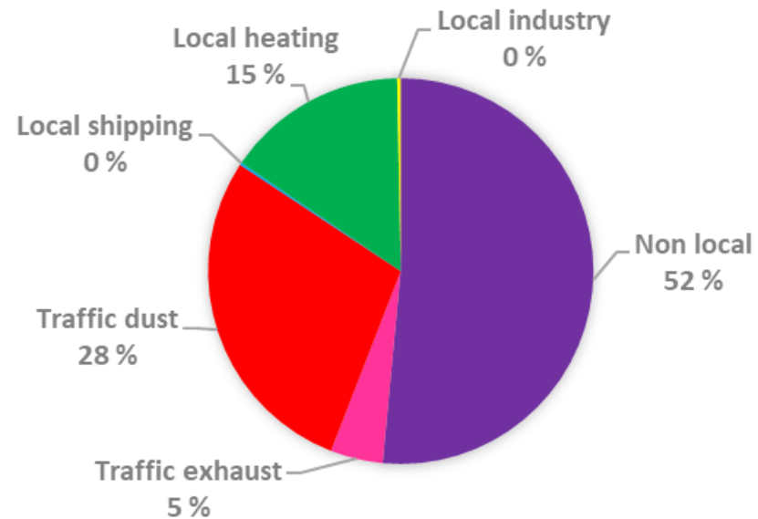
PM 10 SOURCE CONTRIBUTION AT MONITORING SITES 2017
