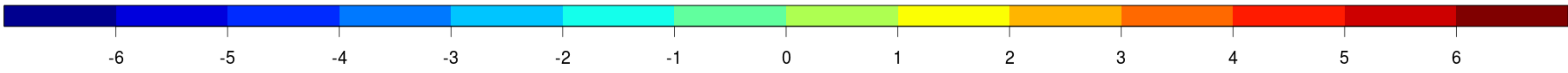
Temperature change (2071-2100 (RCP4.5) vs. 1971-2000) [K] | Top: Raw | Bottom: Bias-corrected (METNO-QMAP-MESAN-1989-2010)
