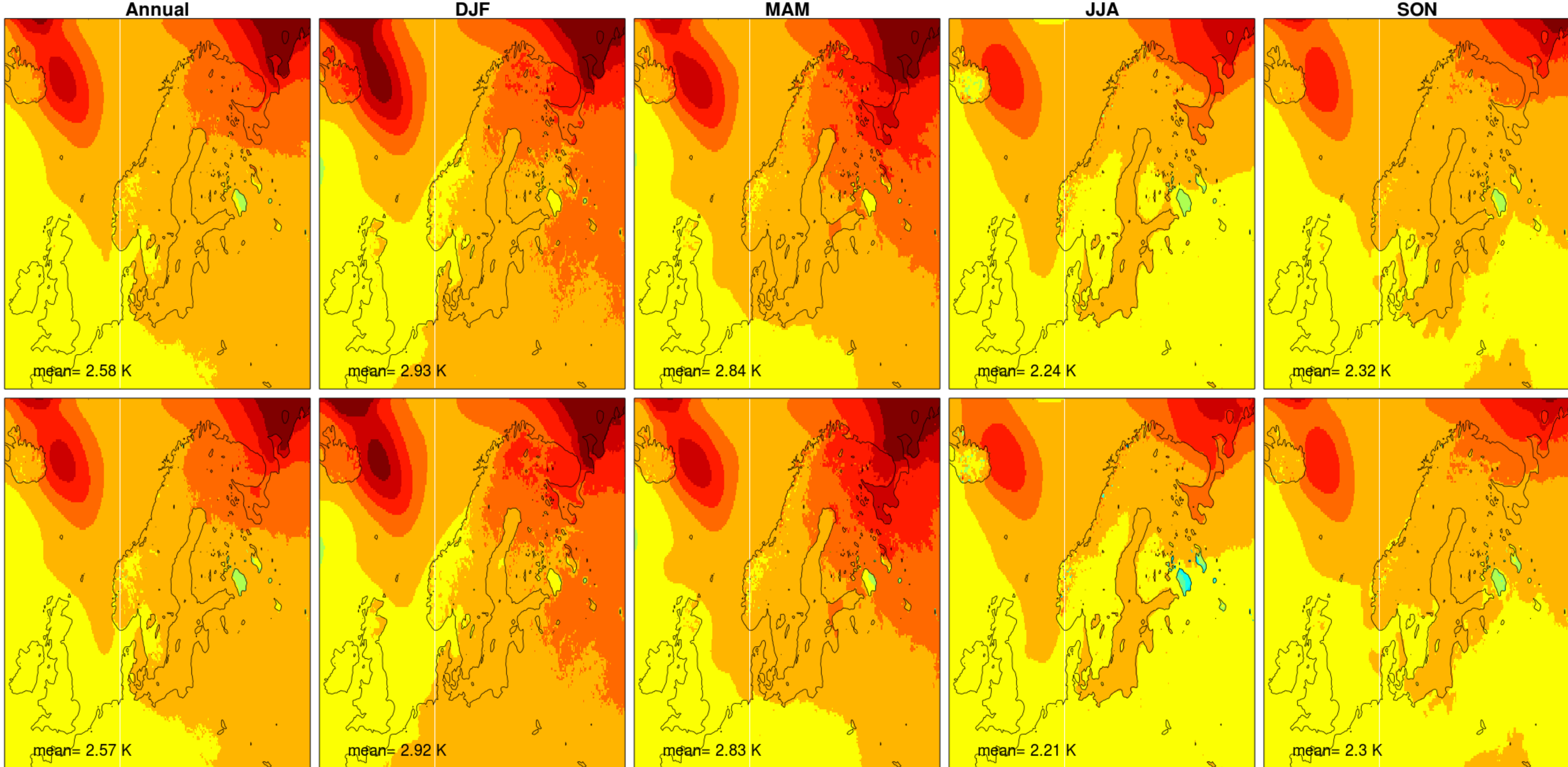
Temperature change (2071-2100 (RCP4.5) vs. 1971-2000) [K] | Top: Raw | Bottom: Bias-corrected (METNO-QMAP-MESAN-1989-2010)
