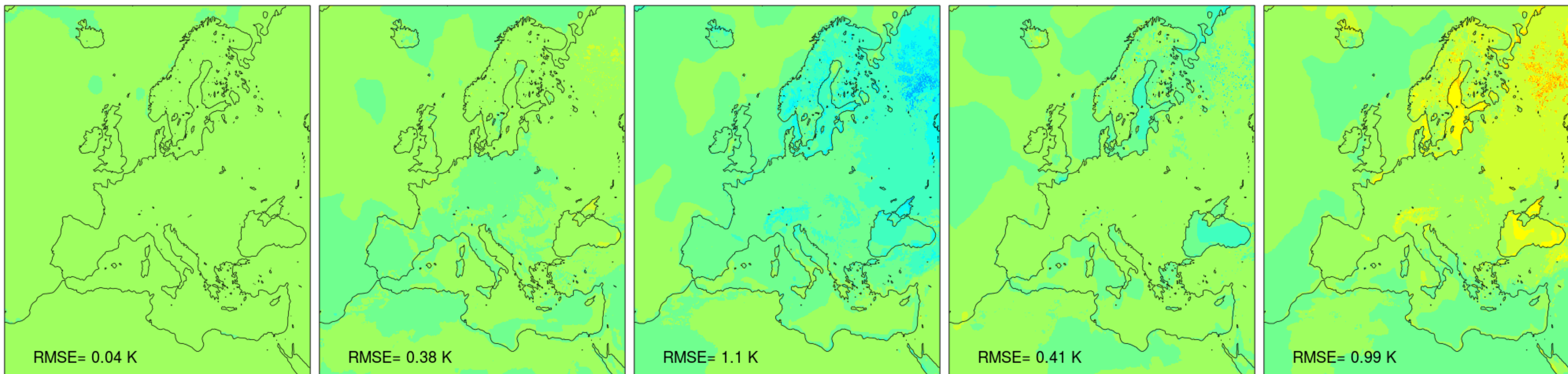
Max. daily temperature bias [K] | Top: Raw | Bottom: Bias-corrected (METNO-QMAP-MESAN-1989-2010)
