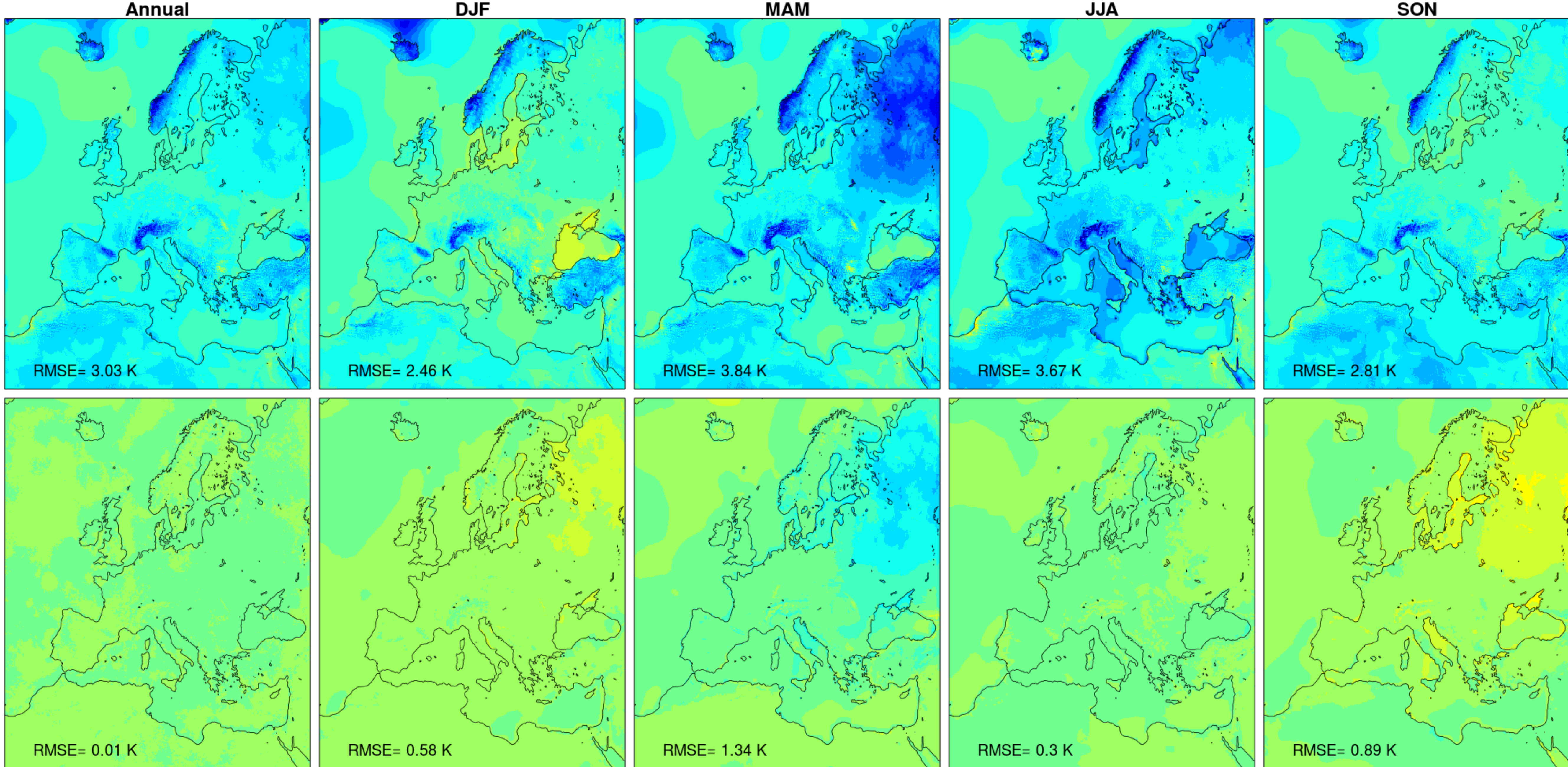
Max. daily temperature bias [K] | Top: Raw | Bottom: Bias-corrected (METNO-QMAP-MESAN-1989-2010)
